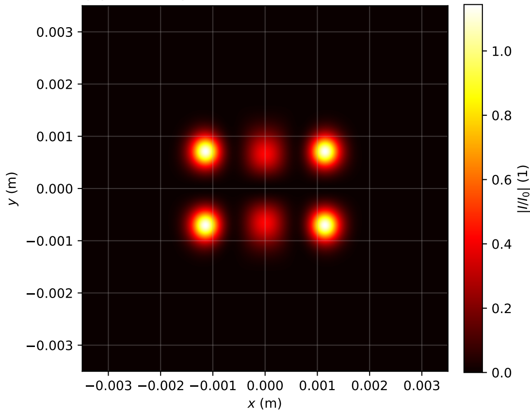
Intensity profile I(x, y, z = 2.070)/I_0 , P_{in}=3.0P_{cr} , artificial time
